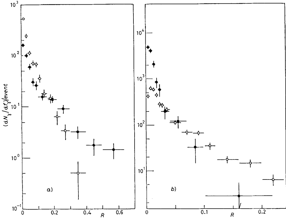
Fig. 8. - Distribution of the fractional energy of gamma-rays, R = f_\gamma = E_\gamma / \sum E_\gamma , for three types of jets: a) ● Mirim jets, ○ Açú jets; b) ○ Açú jets, ● Guaçu jets (1) .
