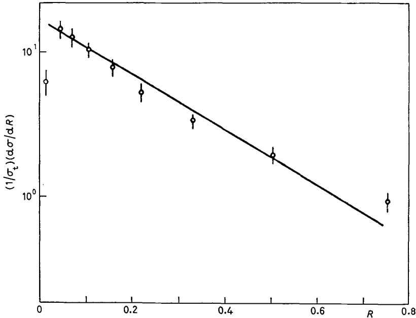
Fig. 9. — Fractional-energy distribution (1/\sigma_t)(d\sigma^{(\pi)}/dR) . Observe that all data points lie on the same curve \propto \exp[-4.3R] . The variable R spans the so-called beam fragmentation region (10) .
