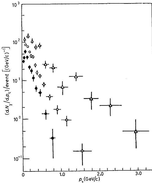
Fig. 1. — Distribution of the \gamma -ray transverse momentum, p_t , for three types of jets: \bullet Mirim jet, \circ Açu jet and \triangle Guaçu jet (1) .
