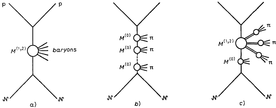
Fig. 7. — a) « peripheral » scheme for the decays into hadrons in the discrete-mass fireball model (see the text), b) the multiperipheral mechanism for the decays into pions, below the M^{(1)} fireball production threshold (see the text), c) above the threshold, the diagram would include also (multiperipheral) production of the M^{(1)} fireball.
