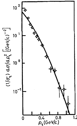
Fig. 10. - Differential p_t^2 distribution for \pi^0 -mesons produced by the Mirim jets (11) : ——— theoretical curve.
