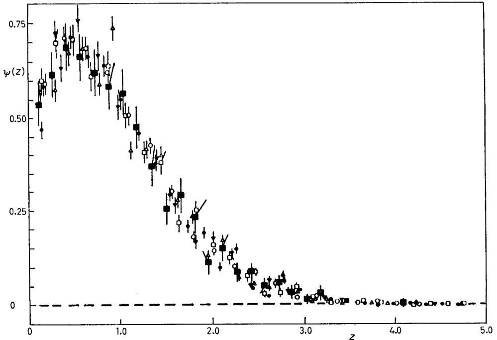
Fig. 6. - The charged-track multiplicity n_{\pm} in the fiducial region. Z = n_{\pm}/\langle n \rangle_{\pm} , \psi(Z) = \langle n \rangle_{\pm} T_n . T_n is the probability for the observation of n tracks and \langle n_{\pm} \rangle = 6.57 is the mean number per event (6). For pp, |\eta| < 1.5 , \sqrt{s} = 23.6 GeV (o), 30.8 GeV (v), 45.2 GeV (□), 53.2 GeV (●), 62.8 GeV (Δ). For p\bar{p} , |\eta| < 1.3 , \sqrt{s} = 540 GeV (■).
