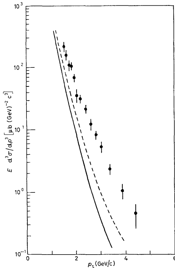
Fig. 2. — † measured invariant cross-section for p\bar{p} \rightarrow \pi^0 + \text{anything} at \sqrt{s} = 540 GeV, — idem , at the ISR energy \sqrt{s} = 53 GeV, — — — extrapolation of data to collider energies using the form E d^3\sigma/dp^3 \sim p_t^{-8}(1-x_t)^9 ; x_t = 2p_t/\sqrt{s} (2).
