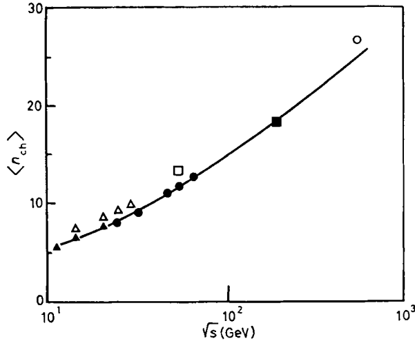
Fig. 4. - Dependence of \langle n_{ch} \rangle upon \sqrt{s} as measured at ISR and lower energies with the fit by THOMÉ et al. (1) \langle n_{ch} \rangle = a + b \log s + c \log^2 s . All inelastic: ● THOMÉ et al. , ■ balloon data (2), ▲ FNAL data (6); nondiffractive: □ UA5 (7), △ FNAL (6), ○ UA5, this experiment. The UA5 data point is for s.d. excluded (4).
