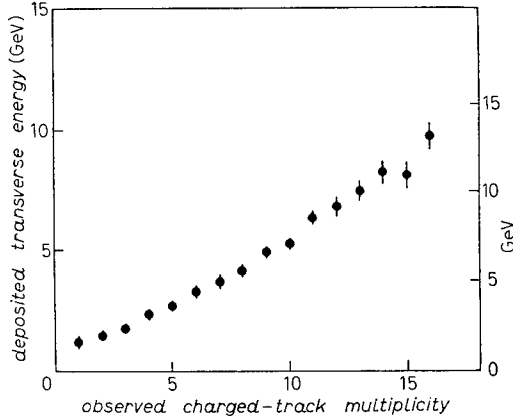
Fig. 5. - Deposited transverse energy as a function of charged-track multiplicity (5).
