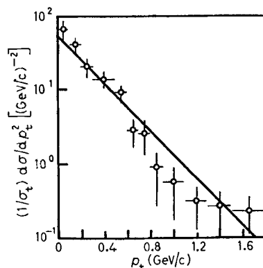
Fig. 11. - Differential p_t^2 distribution for \pi^0 -mesons produced in the Açu jets (11): — kT \sim 0.4 GeV.
