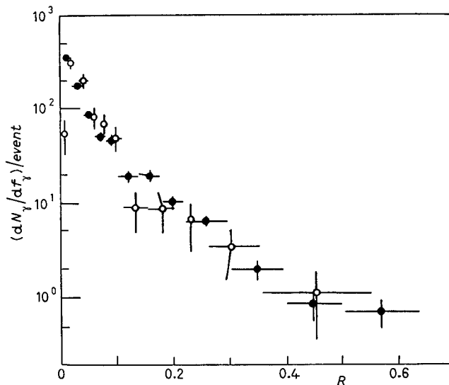
Fig. 3. — Distribution of the fractional energy of \gamma -rays, R = f_\gamma = E_\gamma / \sum E_\gamma : ● 80 Chacaltaya C-jets with \sum E_\gamma > 20 TeV, ○ 9 C-jets by proton primary in balloon experiments, with 2 < \sum E_\gamma < 5 TeV (3) .
